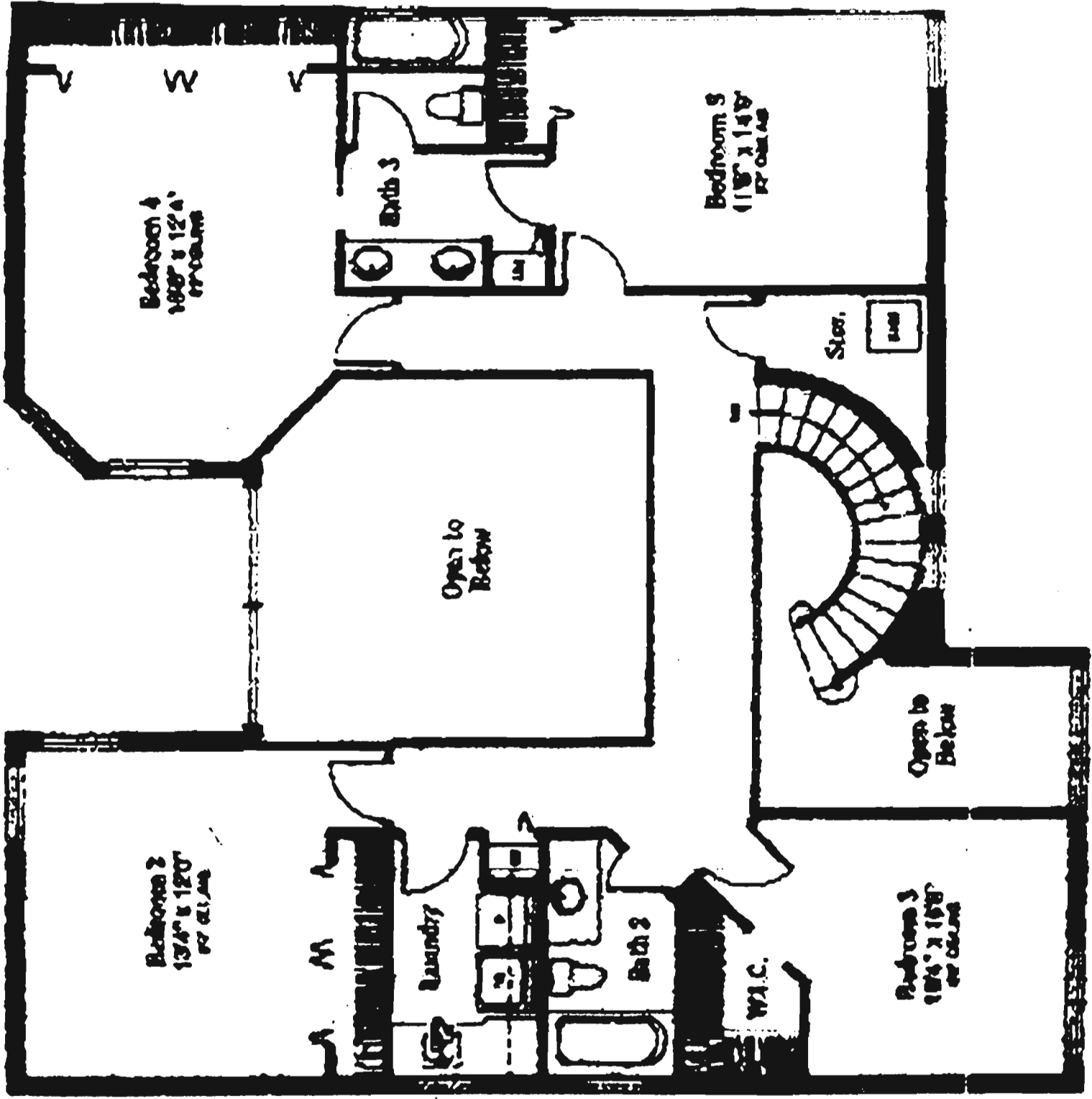
SECOND FLOOR
