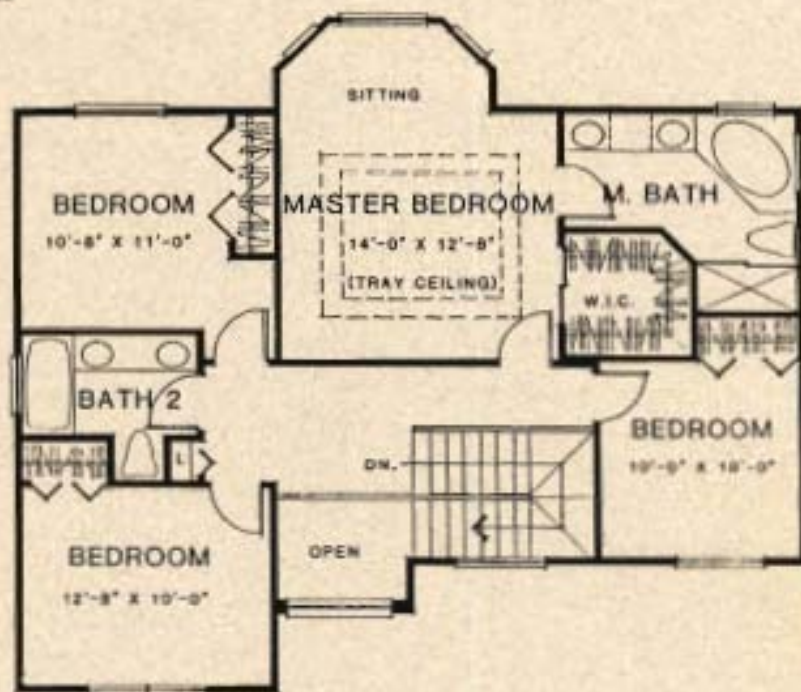
SECOND FLOOR 8'-0" Ceiling throughout except Master Bedroom
